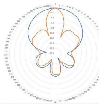
2.4 GHz Antenna Radiation Pattern
