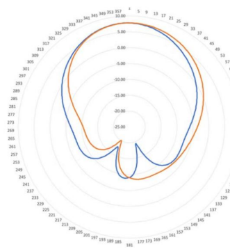
2.4 GHz Antenna Radiation Pattern
