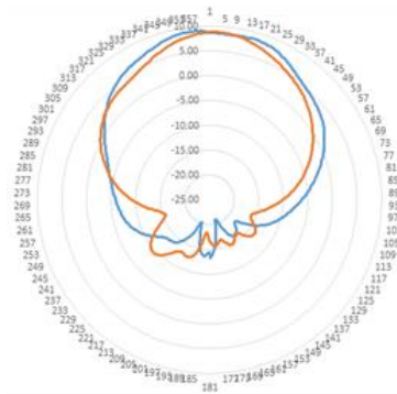
5 GHz Antenna Radiation Pattern
